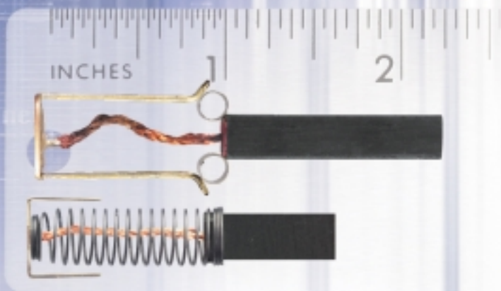
Phoenix Constant Force Cartridge Brush Holder ® (constant force spring)
